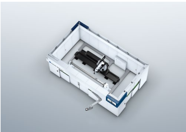
XXL parts are handled by the turnover positioner: the robot moves along a linear axis for further reach.
